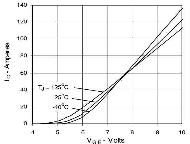
Fig. 6. Input Admittance
