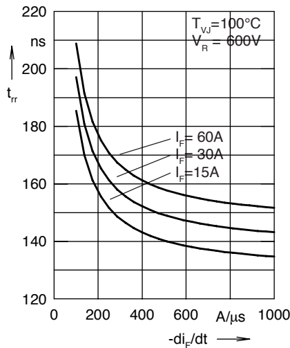
Fig. 28. Recovery time t_{rr} versus -di_F/dt
