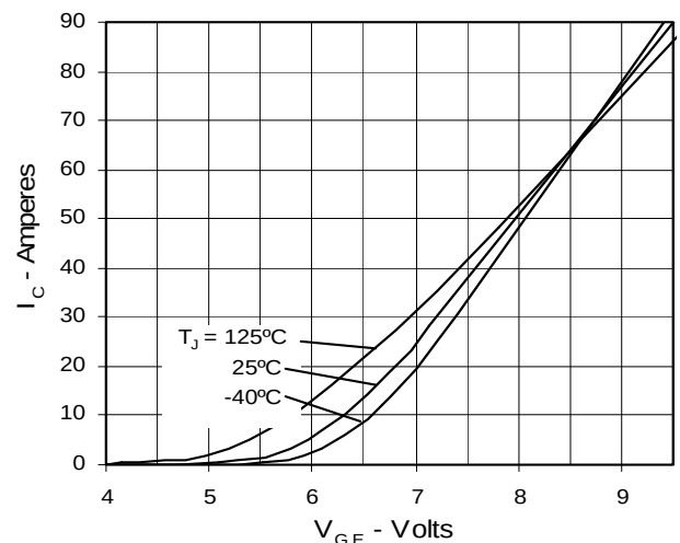
Fig. 6. Input Admittance
