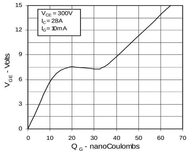
Fig. 14. Gate Charge
