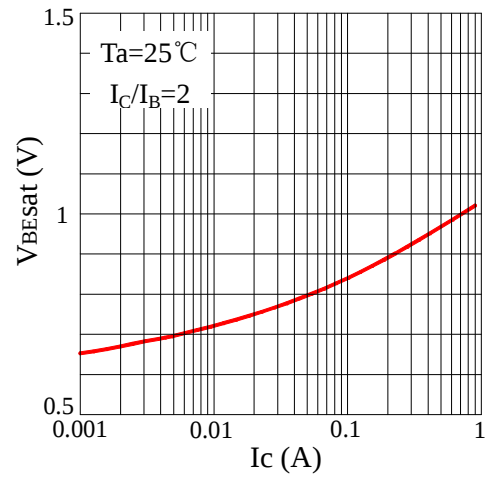
Fig4 V_{BESat}-I_C
