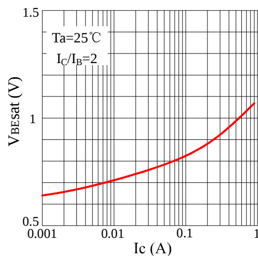
Fig4 V_{BEsat} - I_C
