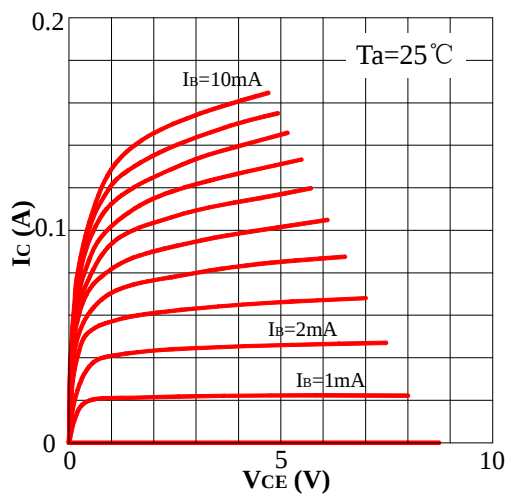
Fig1 Static Characteristic
