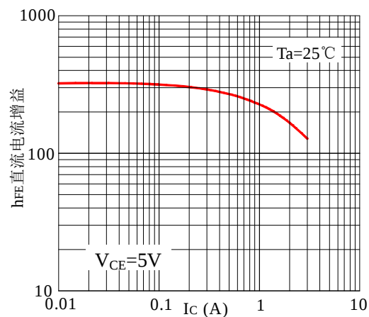
Fig4 hFE-IC
