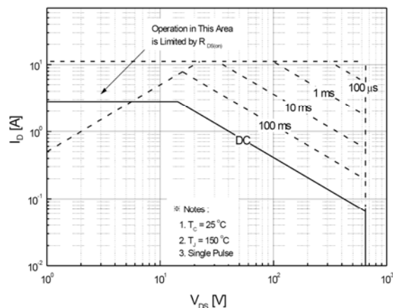
Maximum Safe Operating Area For JCS4N65FC
