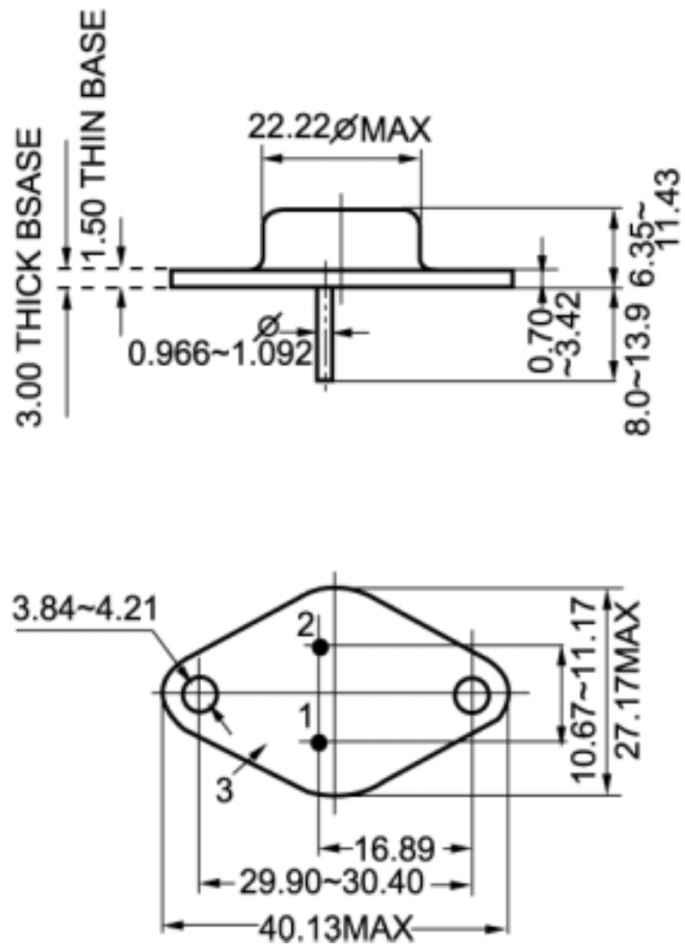
Fig.2 Outline dimensions
