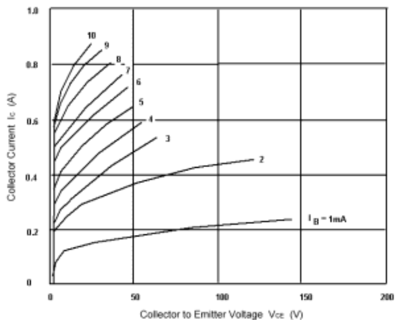
Fig.4 Static Characteristic
