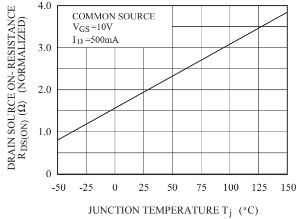
R_{DS(ON)} - T_j
