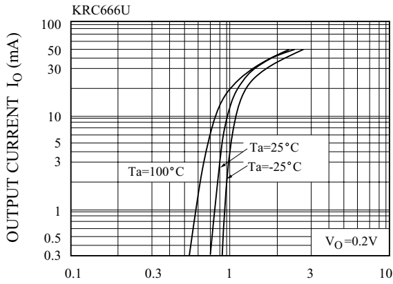
I_O - V_{I(ON)}
