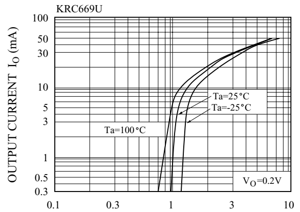
I_O - V_{I(ON)}
