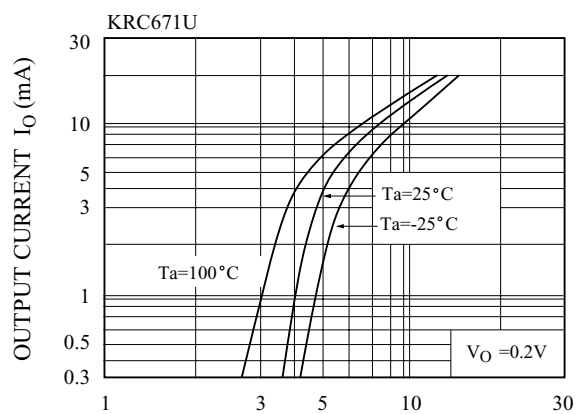
I_O - V_{I(ON)}
