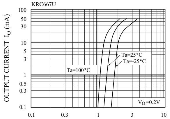
I_O - V_{I(ON)}
