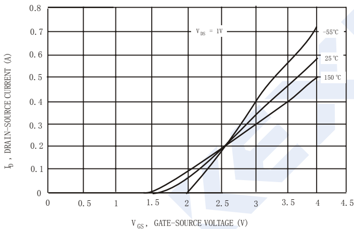
Fig. 2 Transfer Characteristics
