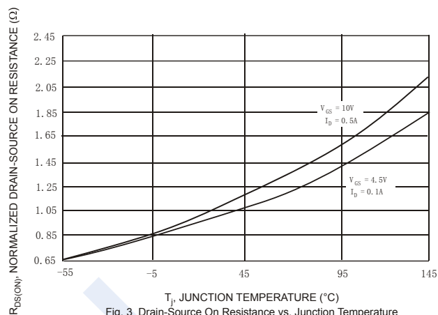
Fig. 3 Drain-Source On Resistance vs. Junction Temperature
