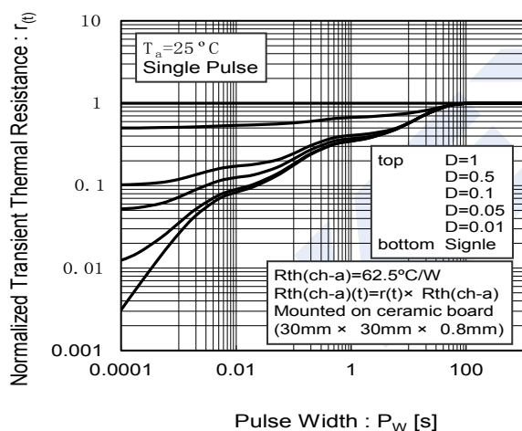
Fig.3 Normalized Transient Thermal Resistance vs. Pulse Width
