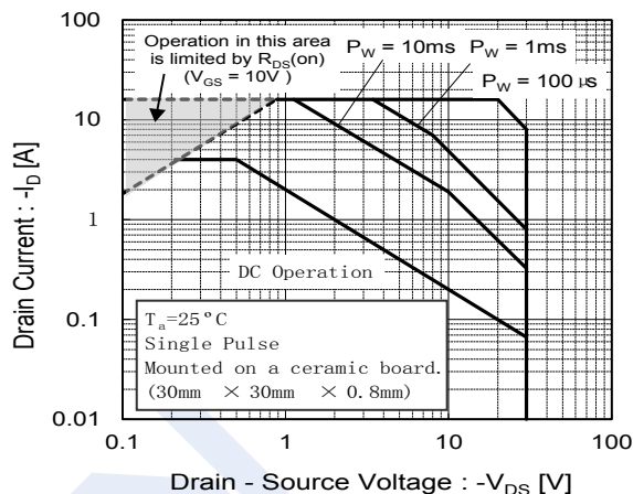
Fig.2 Maximum Safe Operating Area
