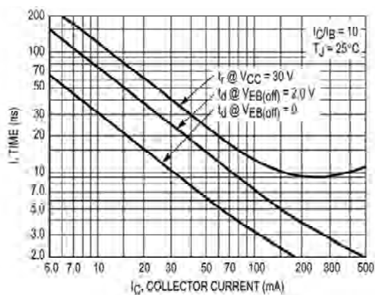
Turn-On Time
