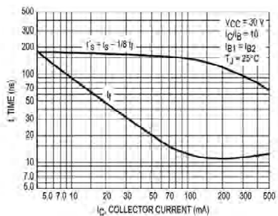
Turn-Off Time
