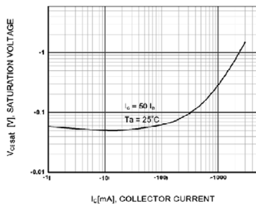
Figure 3. Collector-Emmitter Saturation Voltage
