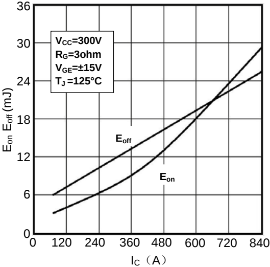
Figure3. Switching Energy vs. Collector Current
