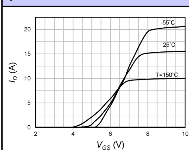
Fig.5 Transfer Characteristics
