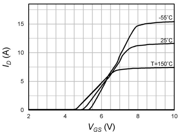
Fig.5 Transfer Characteristics
