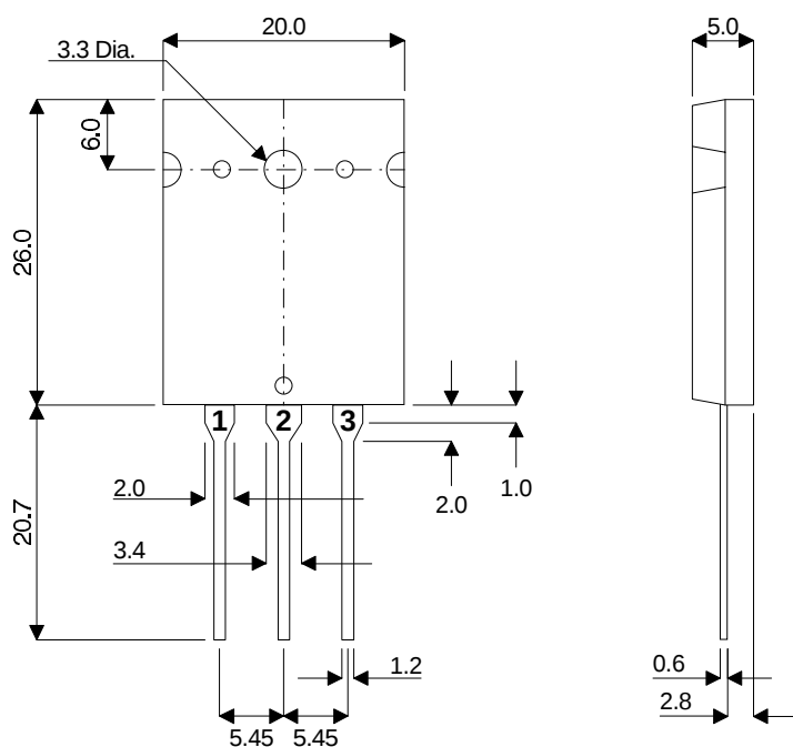
TO-3PBL
