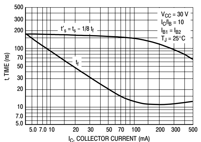
Figure 4. Turn-Off Time
