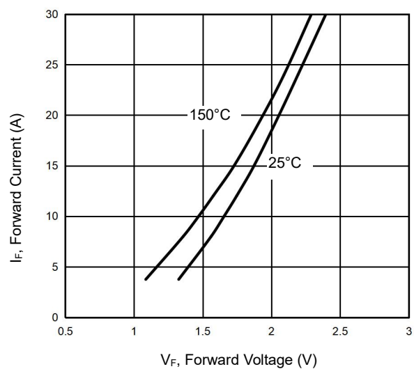
Figure 13 Forward Characteristics
