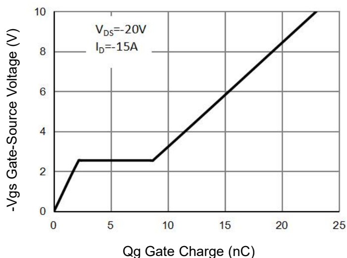
Figure 11 Gate Charge
