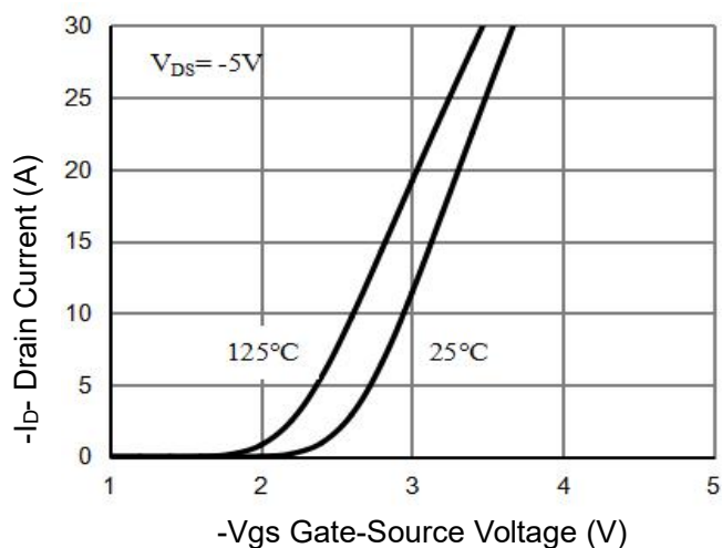
Figure 7 Transfer Characteristics
