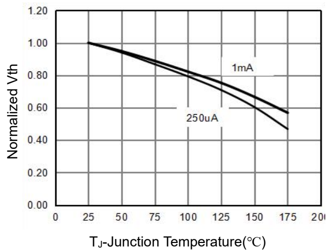
Figure 12 Vth-Junction Temperature
