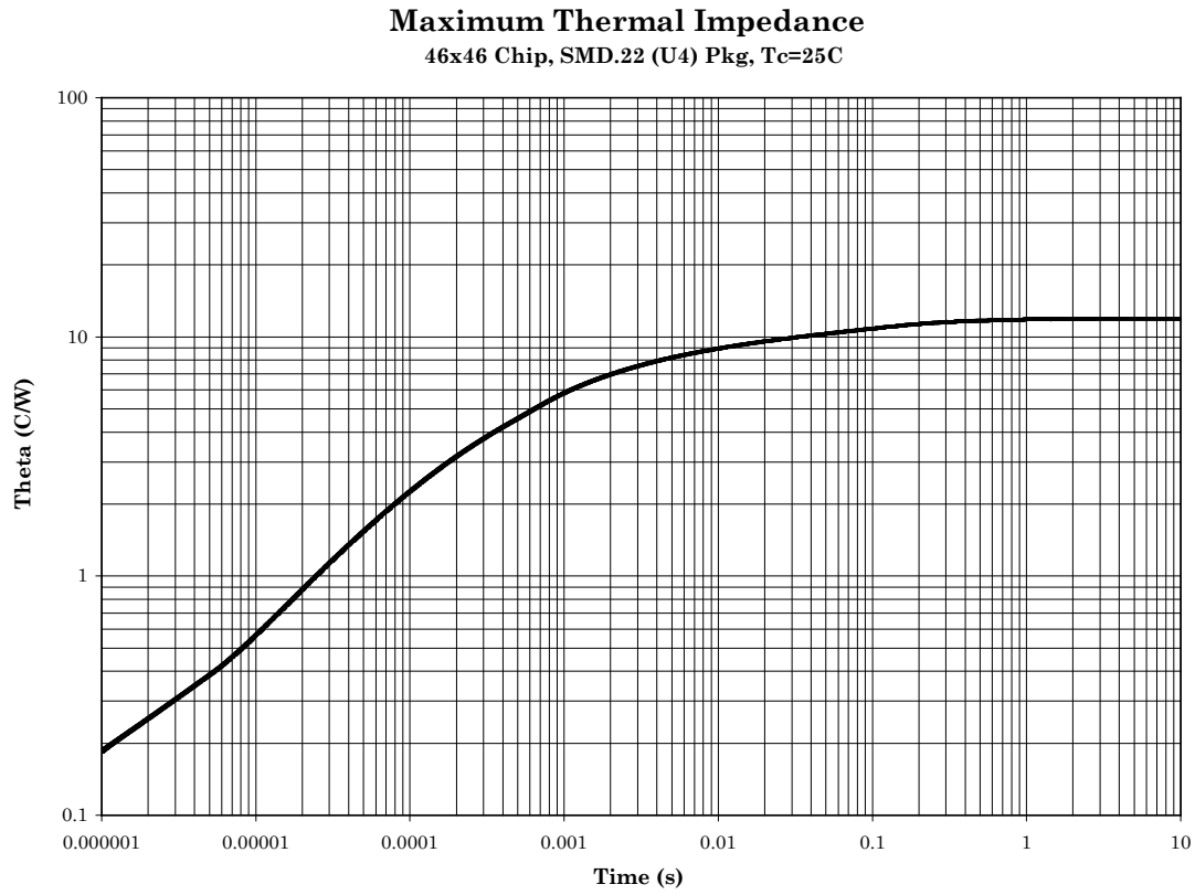
FIGURE 6. Thermal impedance graph ( R_{\theta JC} ) for 2N54115 and 2N5416 (U4).
