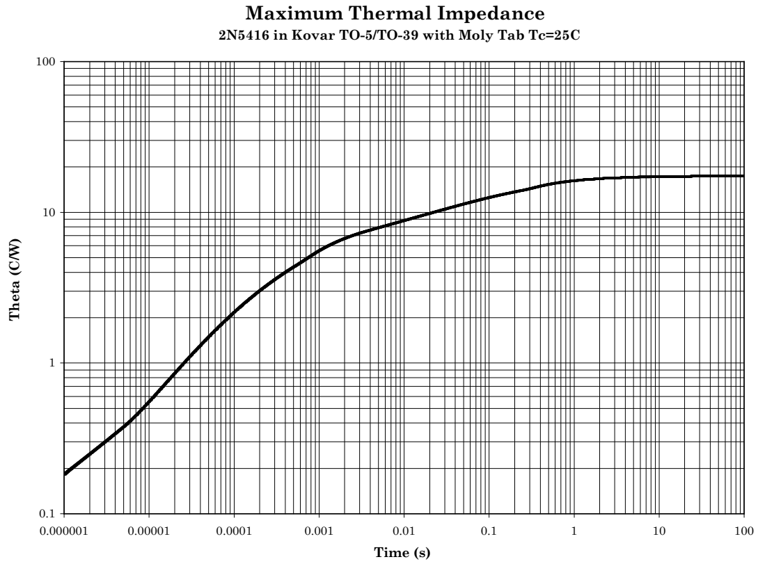
FIGURE 7. Thermal impedance graph ( R_{\theta JC} ) for 2N54115 and 2N5416 (TO-5).
