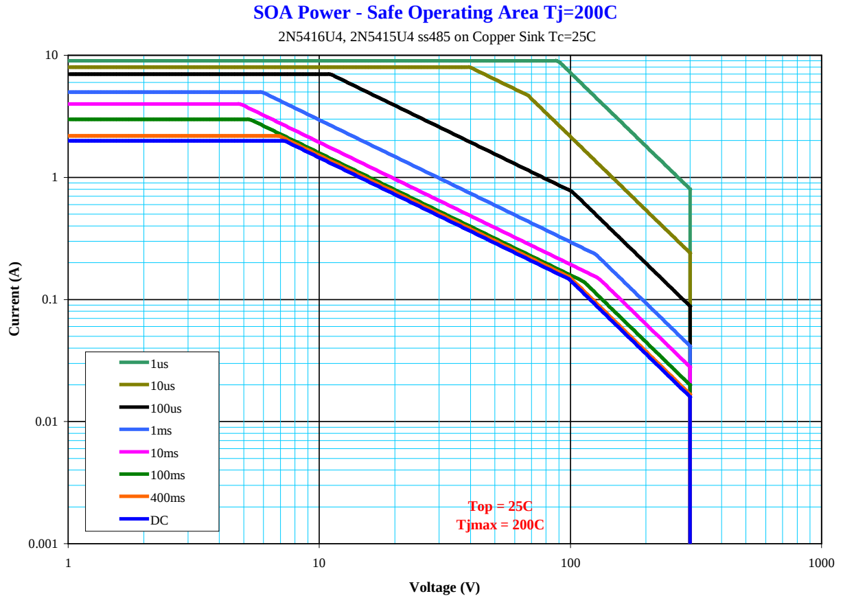
FIGURE 12. Maximum safe operating graph (continuous dc).
