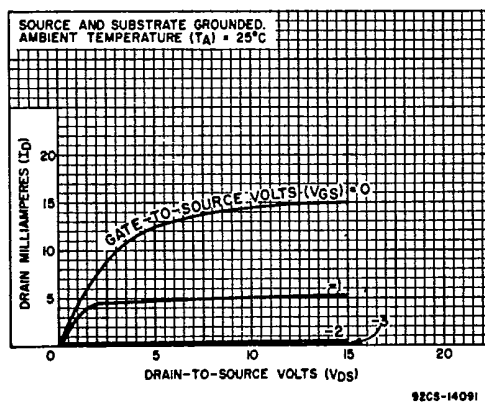
Fig. 6 - Drain Current vs Drain-to-Source Voltage.
