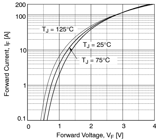
Figure 19. Forward Characteristics
