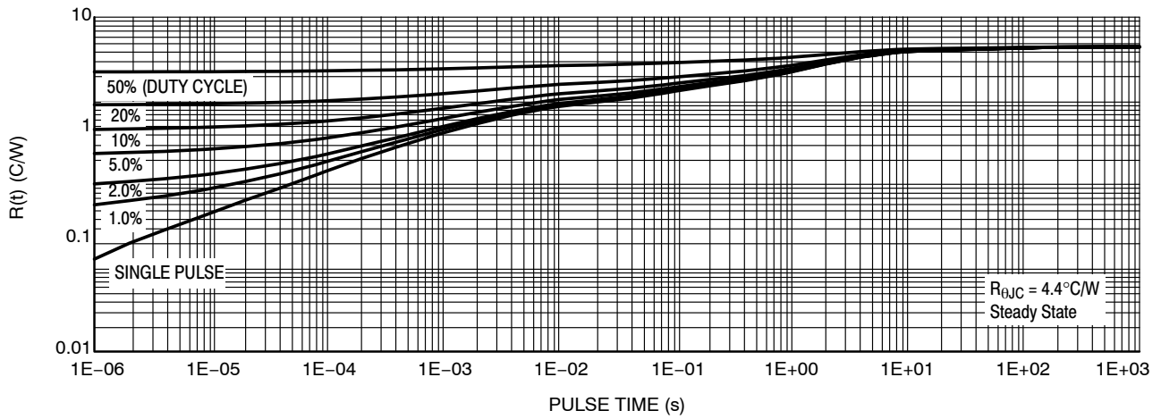
Figure 12. Thermal Impedance (Junction-to-Case) for NDF05N50Z
