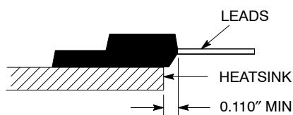
Figure 15. Mounting Position for Isolation Test
