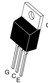
TO-220 CASE 221A STYLE 4
