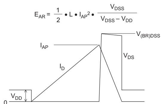
Avalanche Waveform
