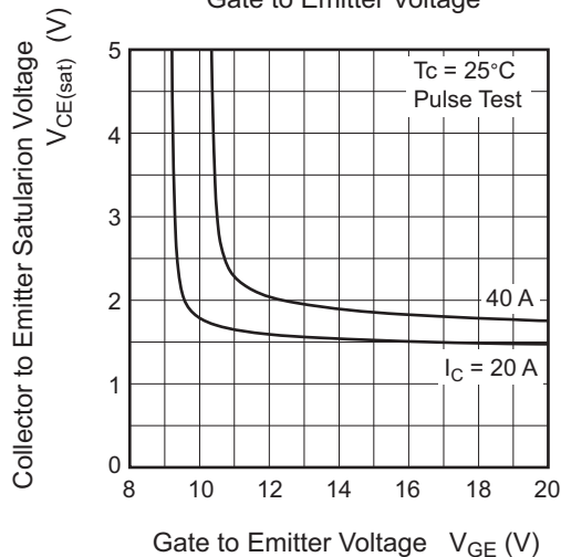
Collector to Emitter Saturation Voltage vs. Gate to Emitter Voltage
