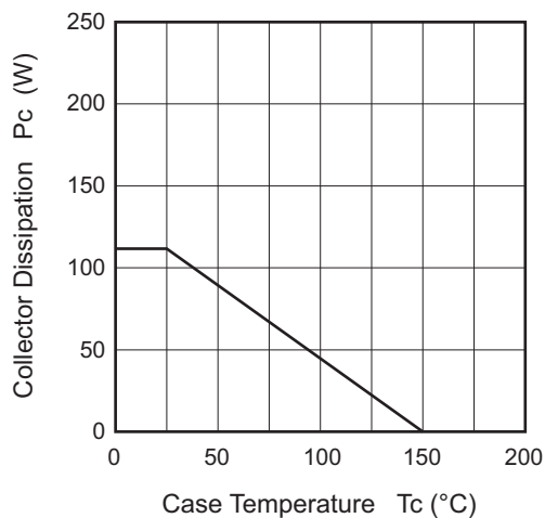
Collector Dissipation vs. Case Temperature
