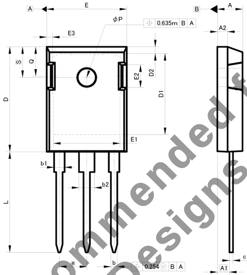
TO-247
