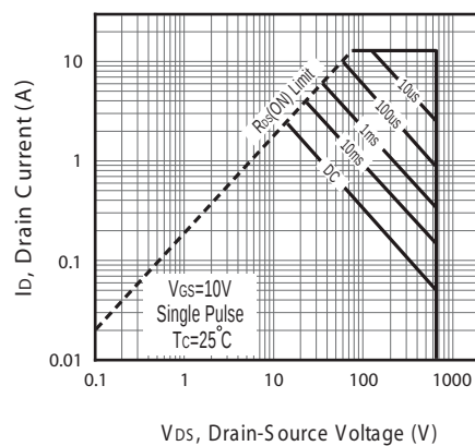
Figure 11b. Maximum Safe Operating Area for SDF04N65
