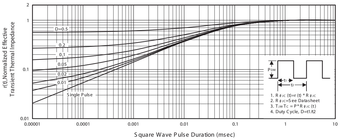
Figure 13b. Normalized Thermal Transient Impedance Curve for SDF04N65
