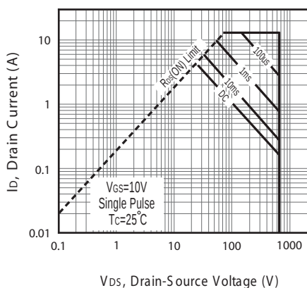
Figure 11a. Maximum Safe Operating Area for SDP04N65
