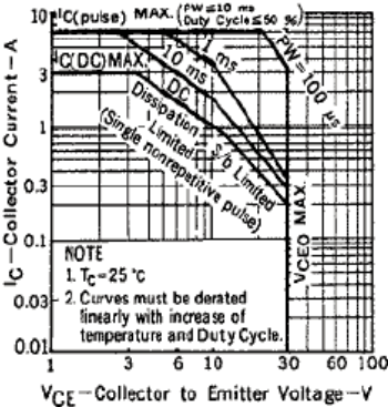
SAFE OPERATING AREAS
