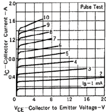
COLLECTOR CURRENT vs. COLLECTOR TO EMITTER VOLTAGE
