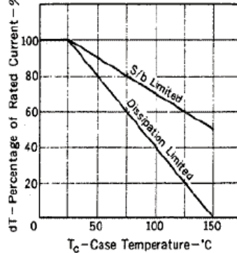
DERATING CURVES FOR ALL TYPES
