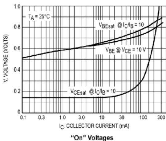
"On" Voltages
