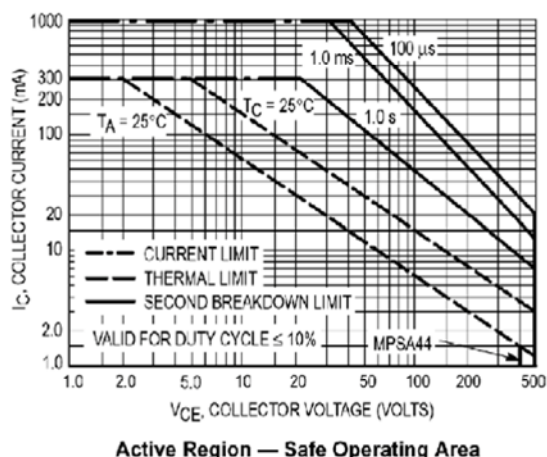
Active Region — Safe Operating Area
