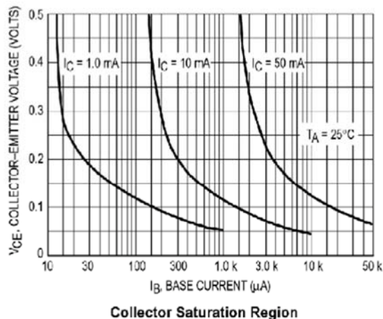
Collector Saturation Region
