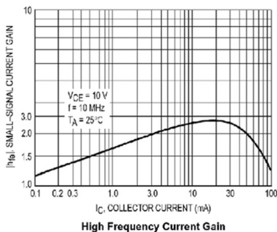
High Frequency Current Gain
