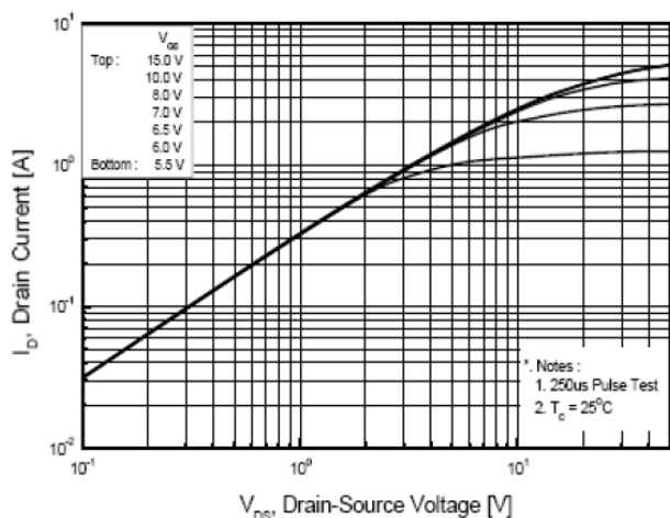
Fig 1. On-State Characteristics
