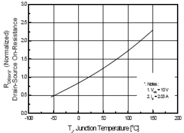
Fig 8. On-Resistance Variation vs. Junction Temperature
