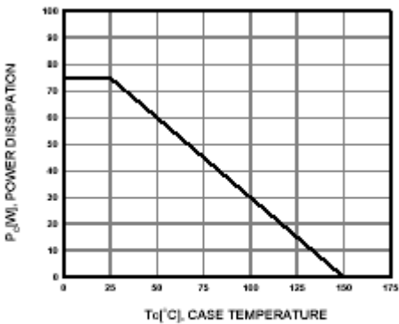
Figure 7. Power Derating
