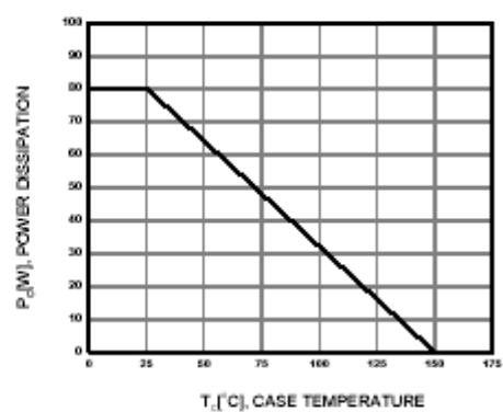
Figure 8. Power Derating
