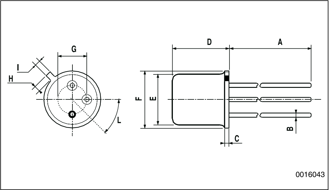
Figure 12. TO-18 drawings
