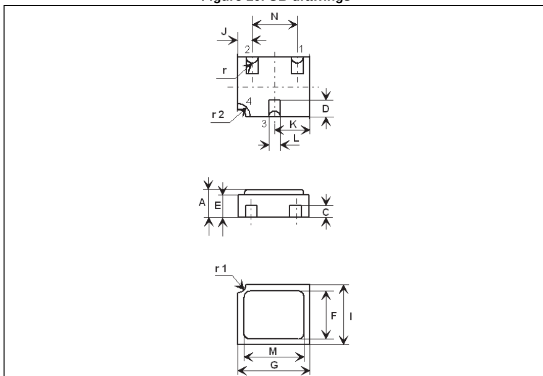
Figure 10. UB drawings
