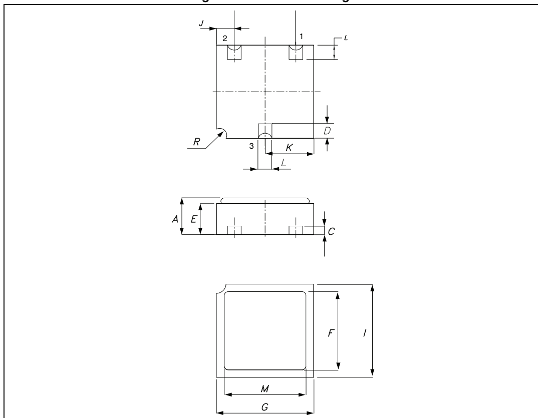
Figure 11. LCC-3 drawings
