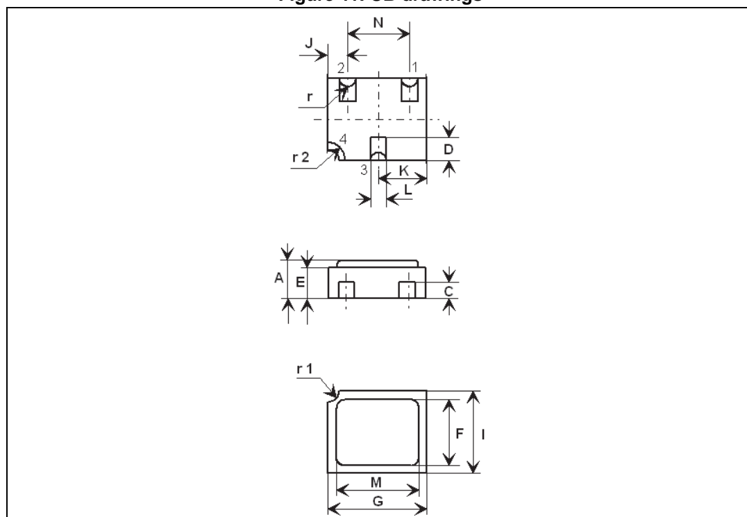
Figure 11. UB drawings
