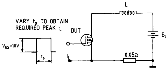
Unclamped inductive test circuit
