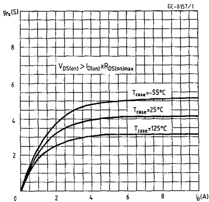
Transconductance
