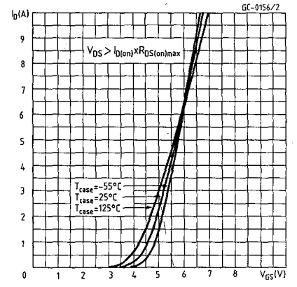
Transfer characteristics
