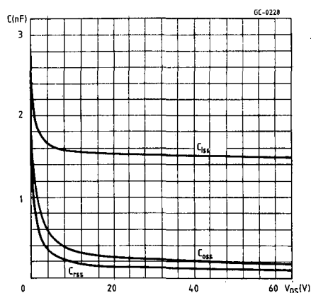
Capacitance variation
