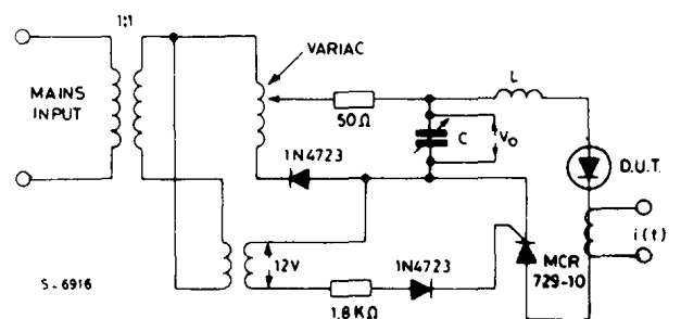
Body-drain diode t_{rr} measurement Jedec test circuit
