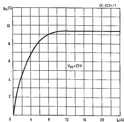
Transconductance
