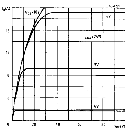
Output characteristics
