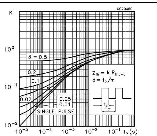
Figure 3. Thermal impedance for DPAK and IPAK
