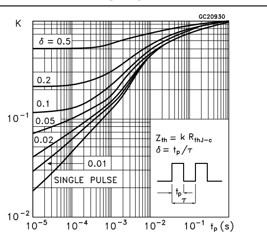
Figure 5. Thermal impedance for D 2 PAK and TO-220
