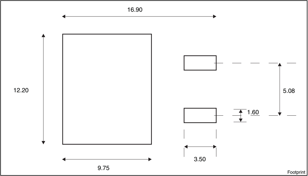
Figure 29. D 2 PAK footprint (a)
