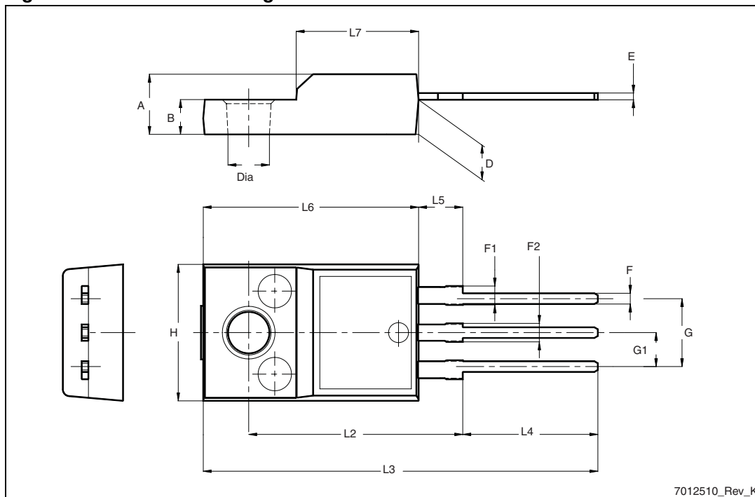
Figure 27. TO-220FP drawing
