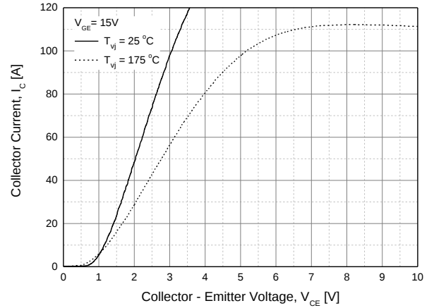
Fig. 2 IGBT Output Characteristics
