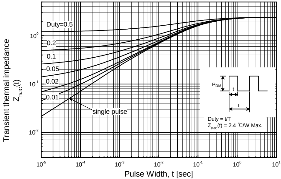
TMP2N60AZ(G)
