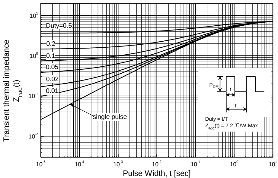
TMPF2N60AZ(G)
