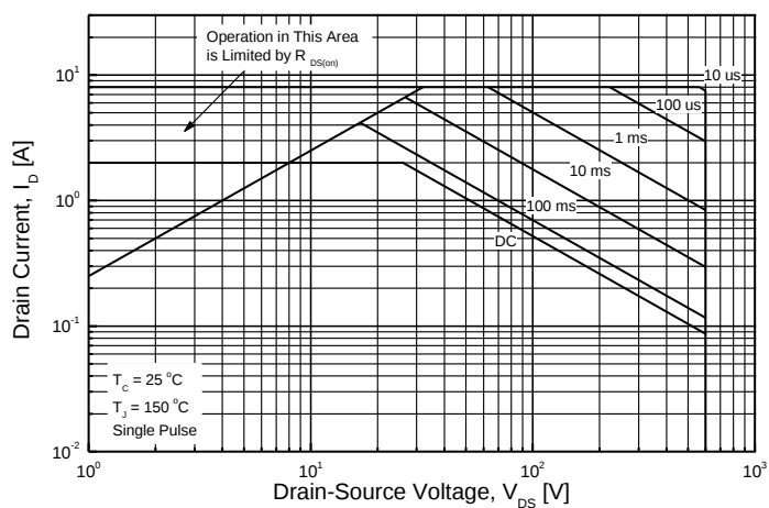
TMP2N60AZ(G)
