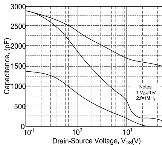
Capacitance Characteristics
