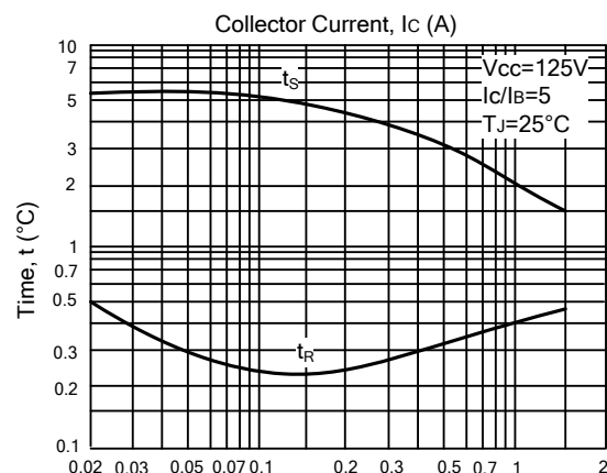
Fig 3. Turn-Off Time
