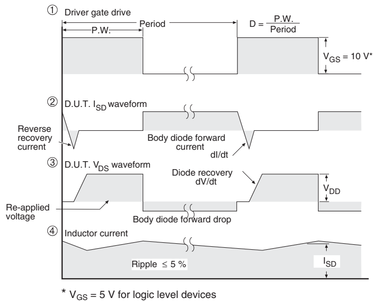
Fig. 14 - For N-Channel
