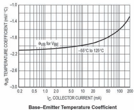
BC546
